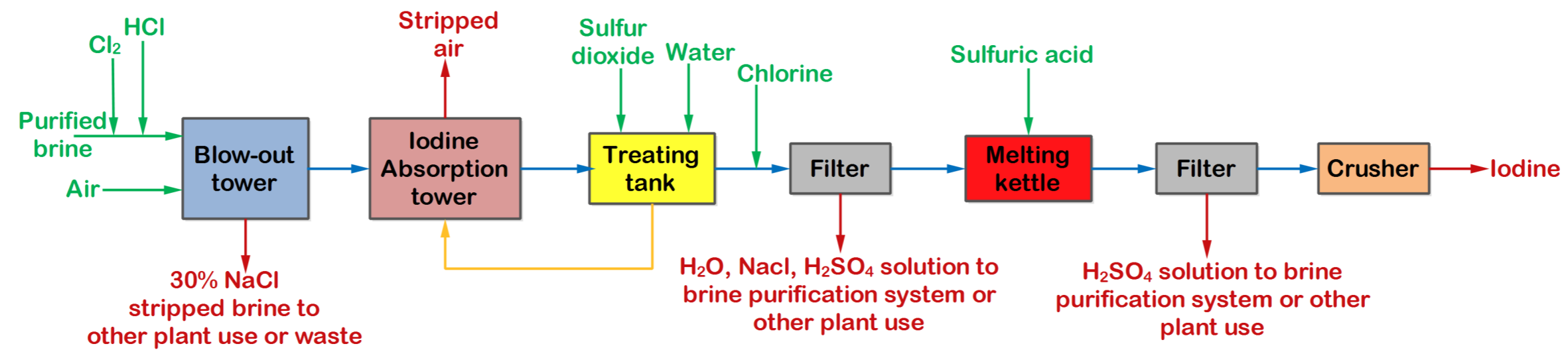
Figure: Manufacture of Iodine from brine and chlorine
